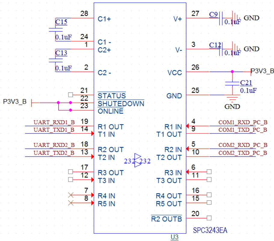
Figure 6. Connections between RS232 COM1, 2 of QD302 and Some Other Devices with an UART / QD302 RS232 COM1、2与其他使用UART接口的设备之间的连接示意图
