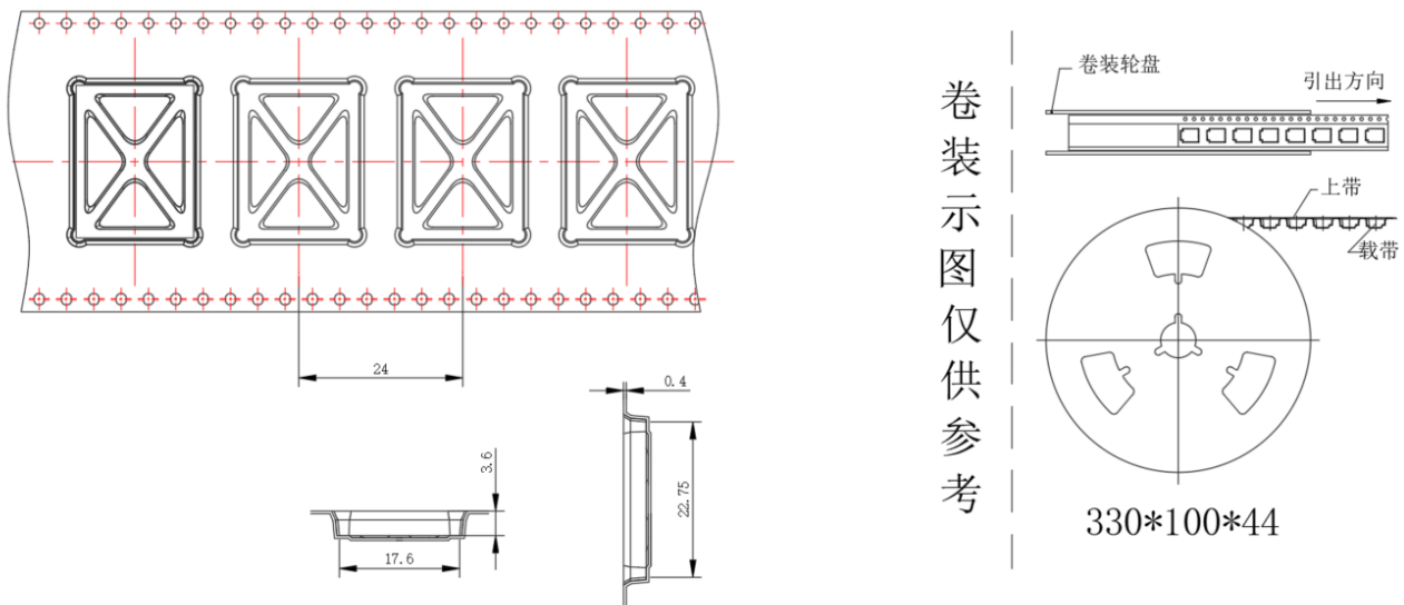
Figure 12. QD302 Roll Tape Packing / QD302卷带包装
