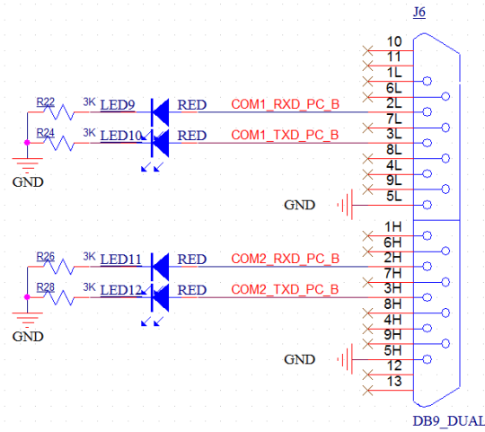
Figure 7. Connection of QD302 COM Connector to PC / QD302 COM与电脑连接原理图
